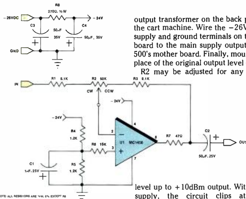
Figure 1. The output buffer stage used for the modification project.
