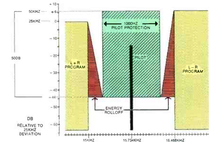
Figure 4. Above, the MTS pilot frequency protection requirements. Note the steep rolloff above 15kHz.
