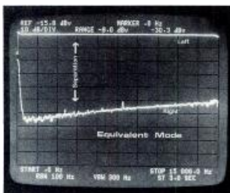
Typical separation performance of a stereo generator switched to the equivalent mode of operation. Separation exceeds 50dB across the audio band (50Hz to 14kHz). The equipment used in this test: a Modulation Sciences TSG stereo generator and SRD-1 stereo decoder and a Hewlett-Packard 3585A low frequency spectrum analyzer/tracking generator.
